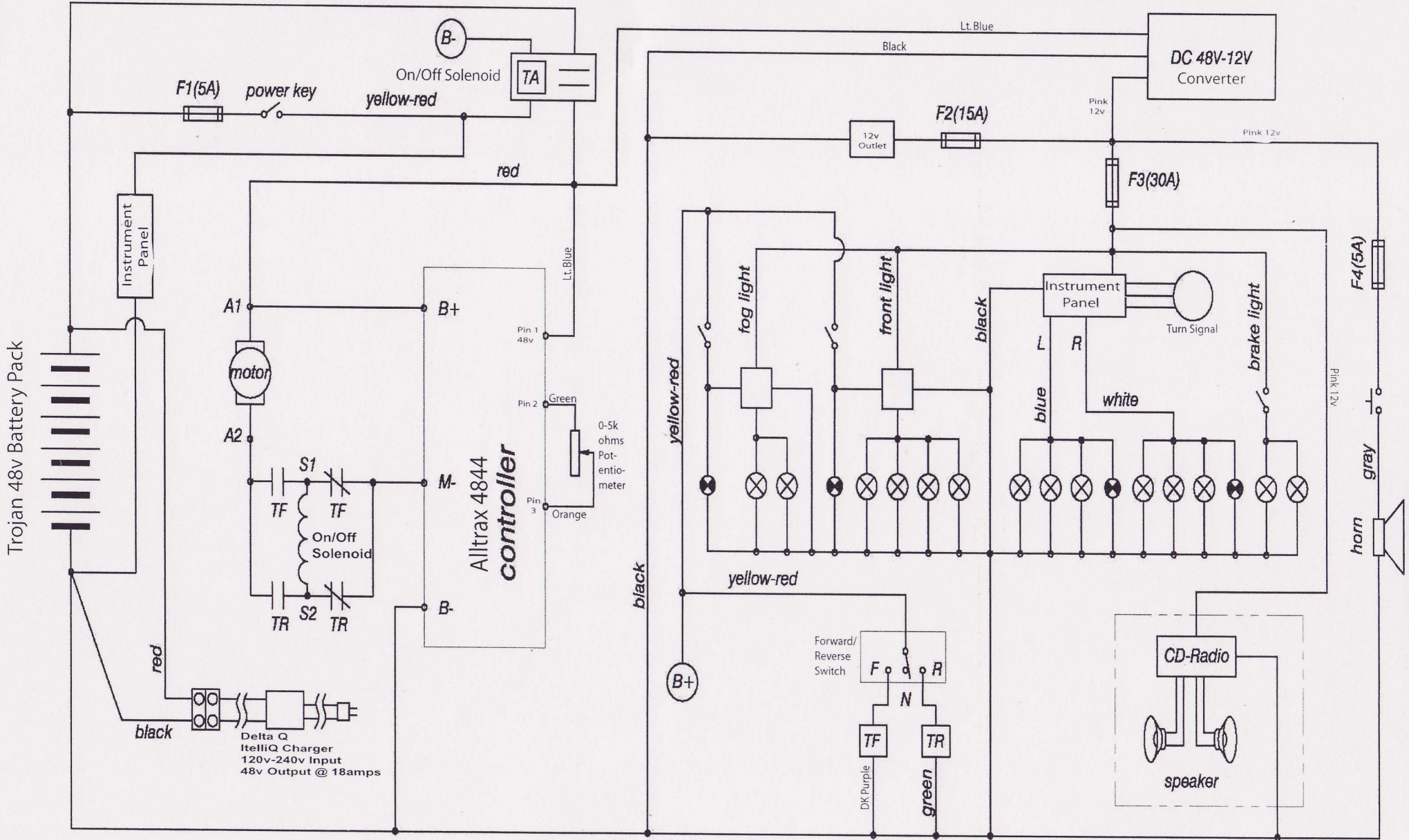
American Custom Golf Cars, Inc. 2006 HUMMER H3 Wiring Diagram
